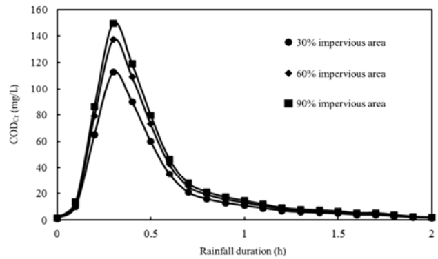
Figure 9. Variation of COD Cr concentration with impermeable area.
